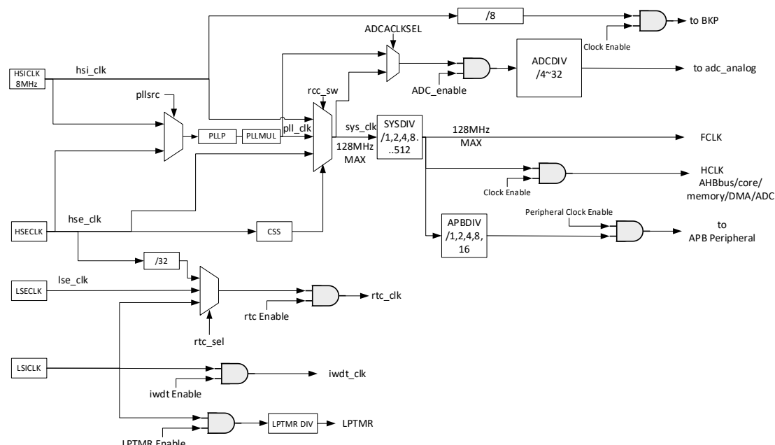
Figure 6 Clock Tree
