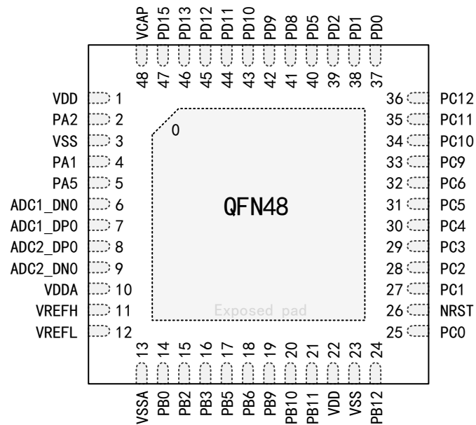
Figure 3 Distribution Diagram of QFN48 Pins
