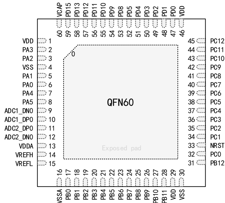
Figure 2 Distribution Diagram of QFN60 Pins
