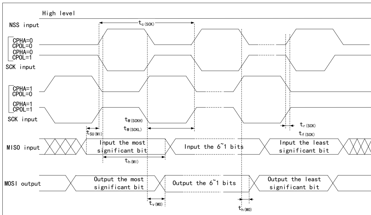
Figure 19 SPI Timing Diagram - Master Mode
